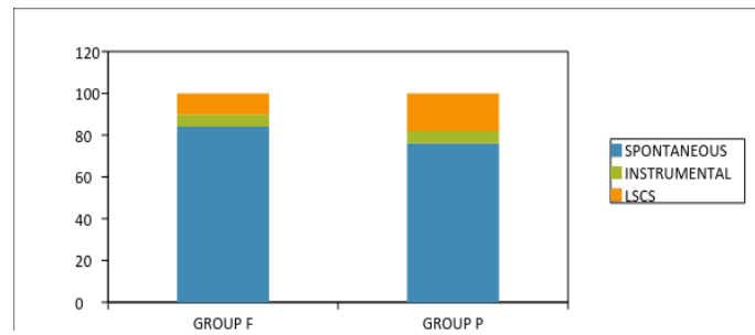
GRAPH 1: Mode of Delivery
