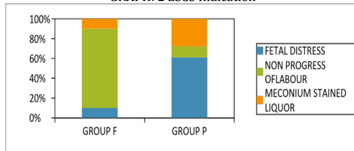
GRAPH: 2 LSCS Indication
